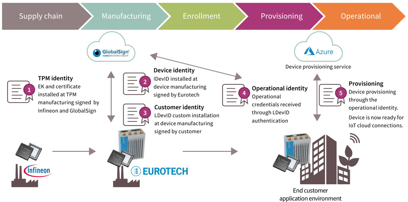
Image 3: Device identities life cycle
