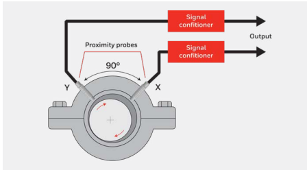
Figure 6: Location of proximity probes [Ref: 9.a]
