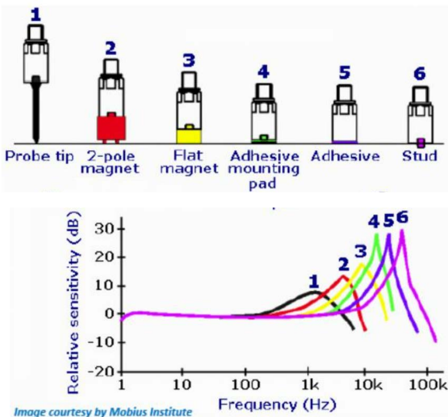
Figure 21: Methods to mount a vibration sensor and its frequency spectrum
