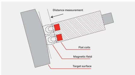
Figure 5: Operating principles of proximity probes [Ref: 9.a]
