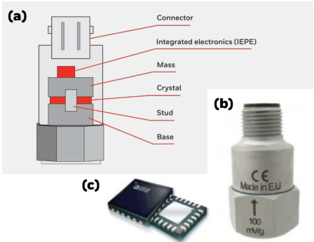
Figure 8: Accelerometer (a) Internal construction (b) Actual representation (c) MEMS type [Ref 9.c]
