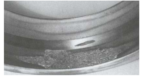
Figure 14: Outer race wear
