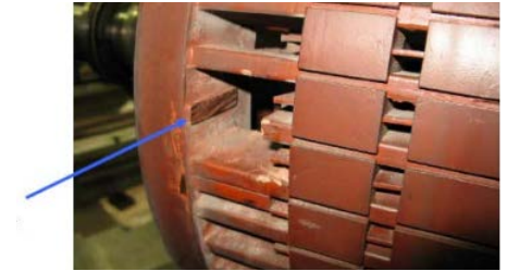
Figure 18: Missing rotor bar [Image ref: 9.i]
