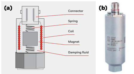
Figure 7: Velocity sensor (a) Internal construction (b) Actual representation [Ref: 9.b]
